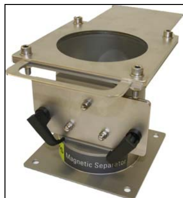
Example EXTRACTOR with slide gate
